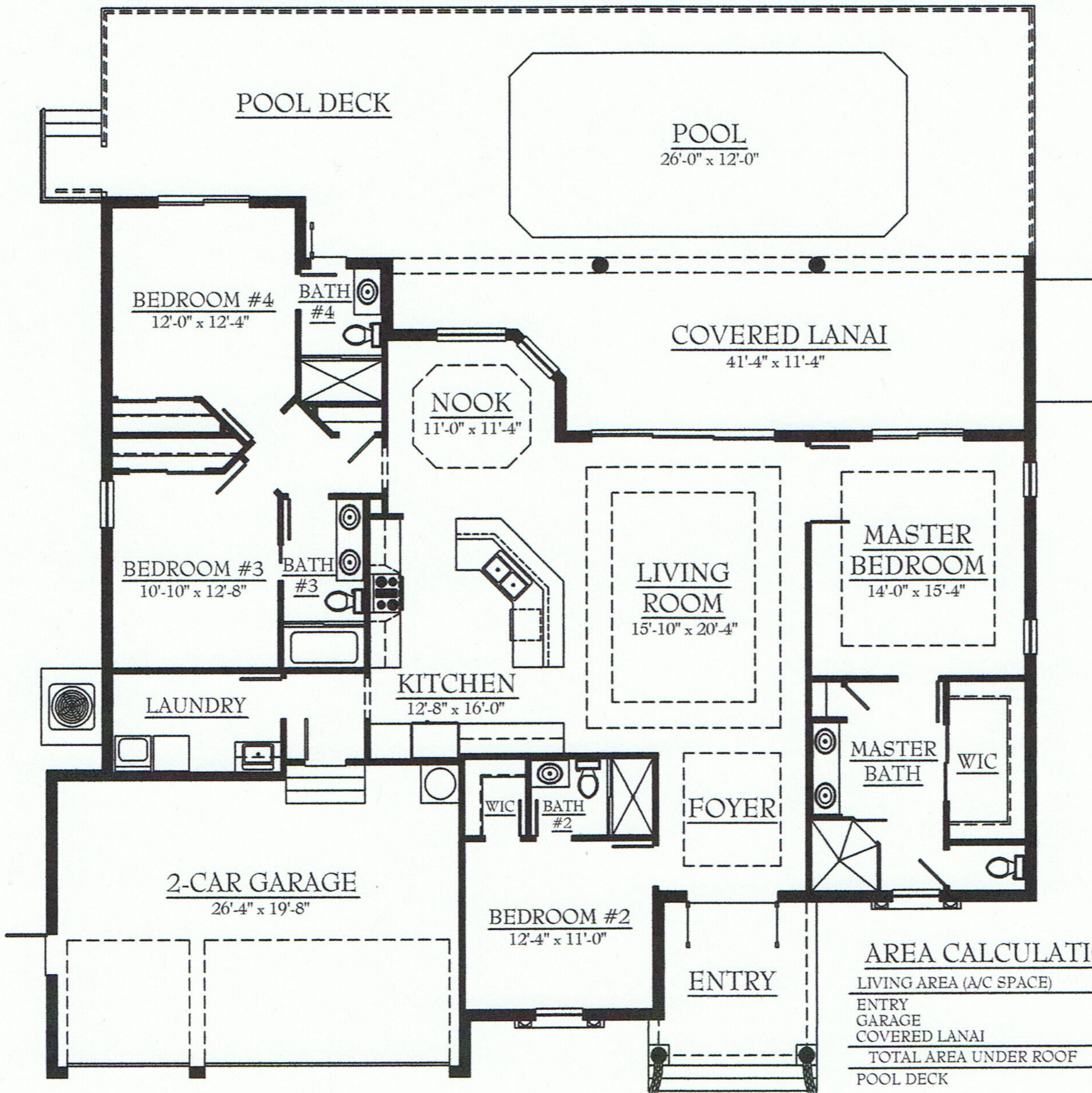
FLOOR PLAN
