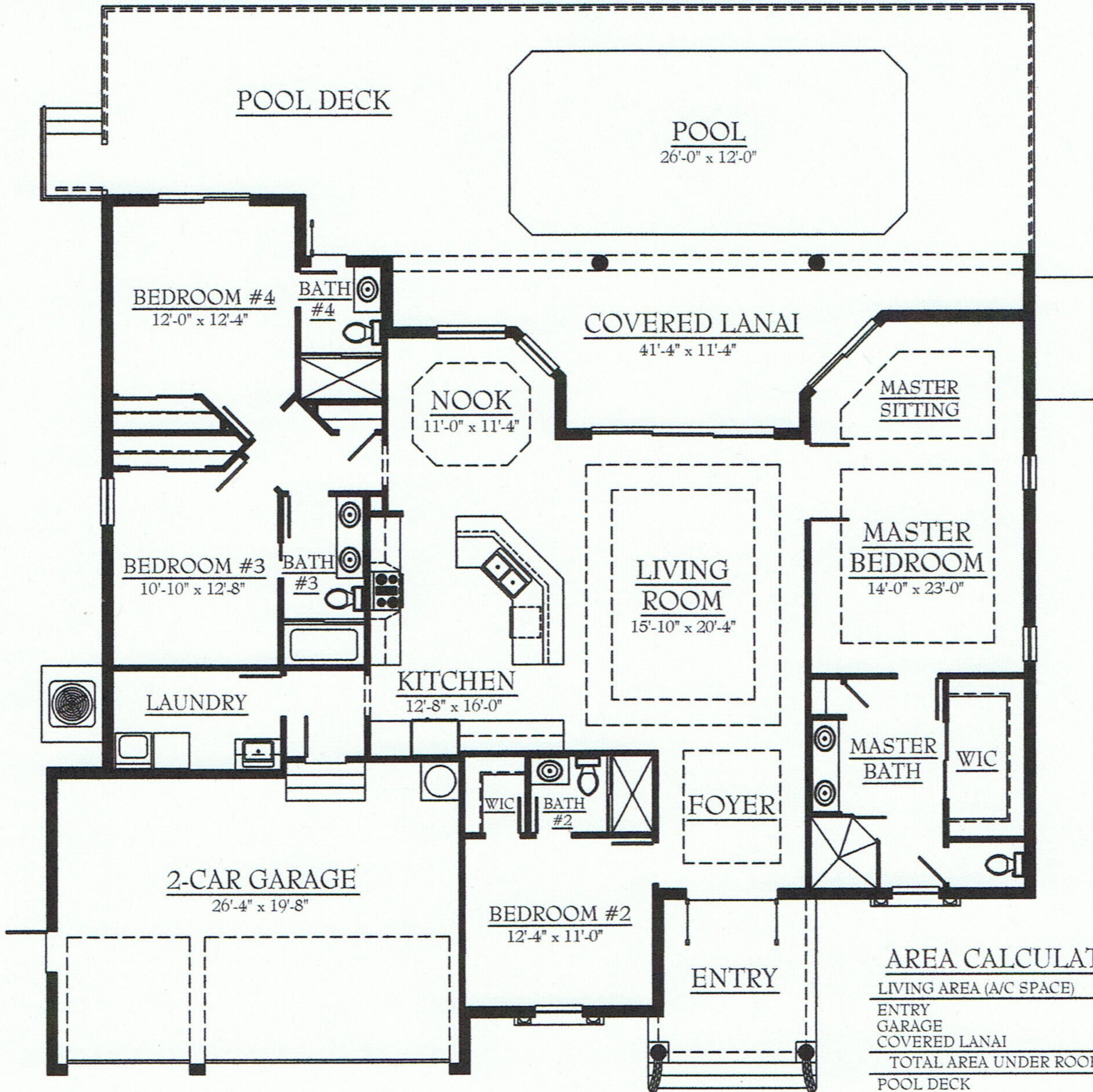
FLOOR PLAN
